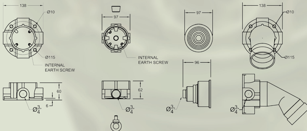
Ceiling Mounting
